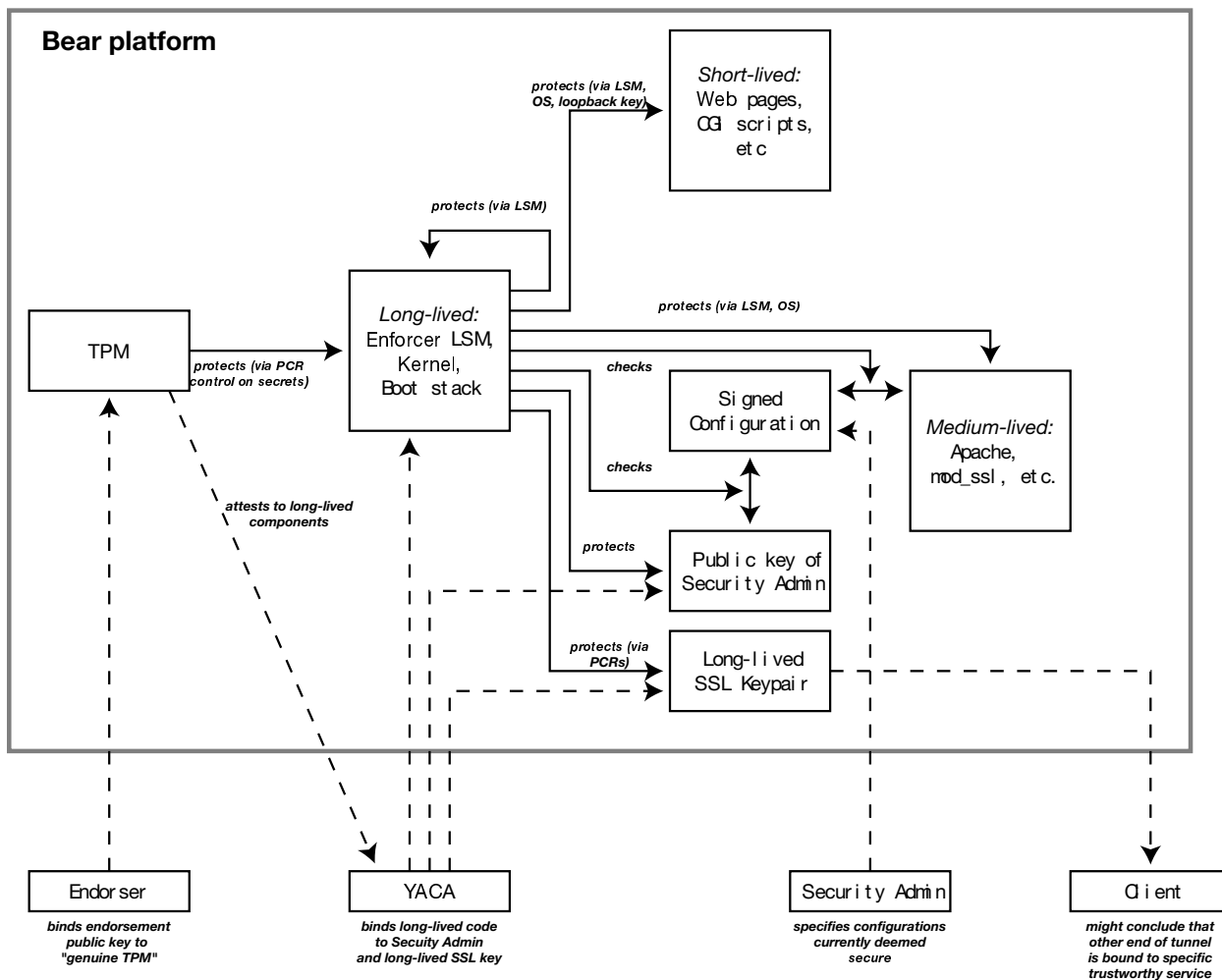
Figure 1: Sketch of the flow of protection and trust in our platform, configured as a Web server. To enable a client to make a trust decision about dynamic content based on a long-lived SSL keypair, we introduce indirection between the core long-lived components and the more dynamic components. Our intention is, like the IBM 4758, the TPM/Linux platform would let the end user buy the hardware, which could authenticate these components to “Yet Another CA.”
