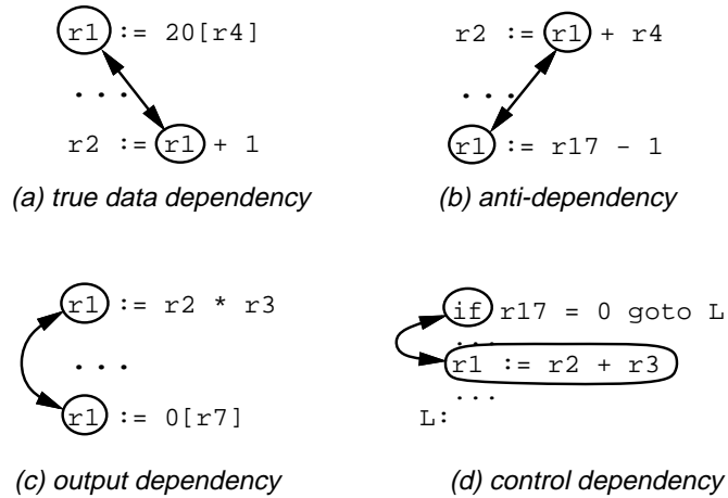
Figure 3: Dependencies
