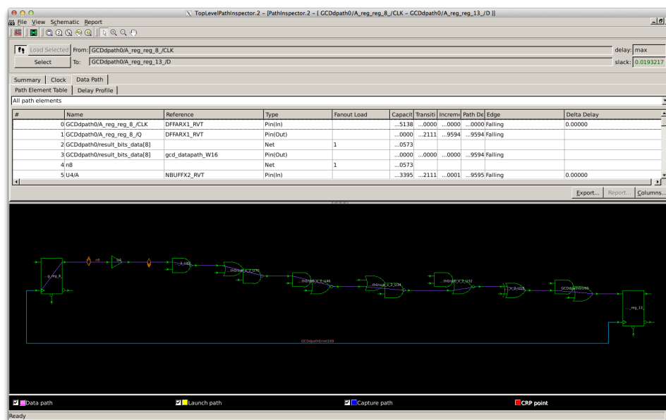
Figure 3: Inspector window showing Data Path tab
