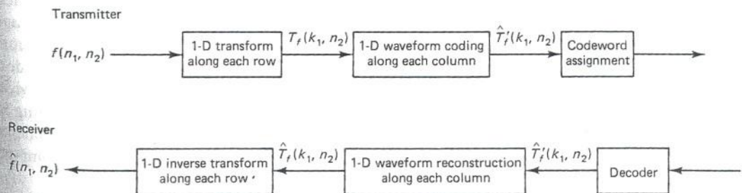
Figure 10.51 Hybrid transform/waveform coder.
