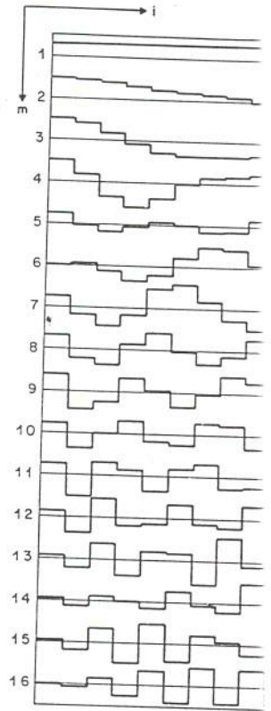
Fig. 5.3.8 KLT basis vectors for the image "Karen" with N=16 and \mu = 0 . For each m the t_m is an
