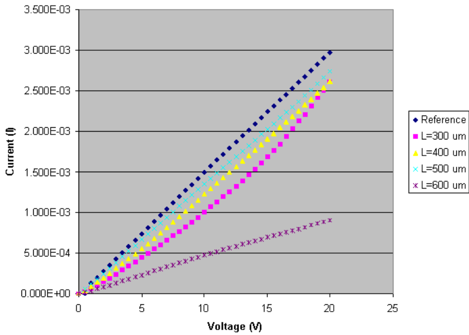
Expected Cantilever I-V Data
