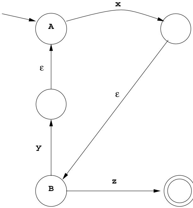
Figure 3.7: Example of converting a regular grammar into a NFA.
