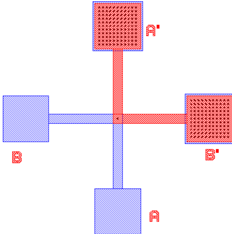
17.(A) METAL-POLY CONTACT RESISTANCE TEST STRUCTURE
