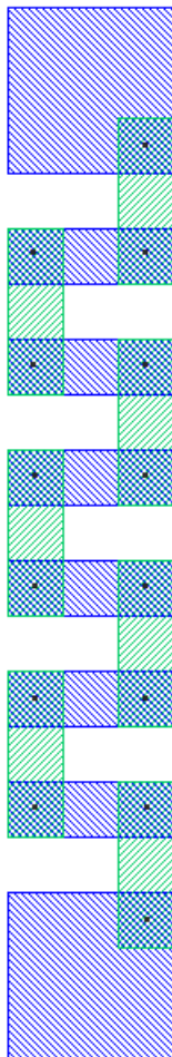
2c metal - diff contact res
