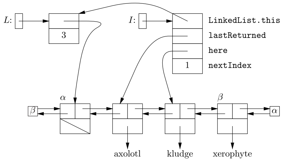
Figure 4.5: A typical LinkedList (pointed to by L and a list iterator (pointed to by I )). Since the iterator belongs to an inner class of LinkedList , it contains an implicit private pointer ( LinkedList.this ) that points back to the LinkedList object from which it was created.
