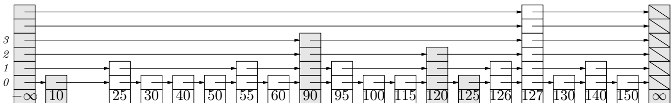
Figure 9.19: The skip list from Figure 9.18 after inserting 127 and 126 (in either order), and deleting 20. Here, the 127 node is randomly given a height of 5, and the 126 node a height of 1. The shaded nodes show which previously existing nodes need to change. For the two insertions, the nodes needing change are the same as the light-shaded nodes that were examined to search for 127 (or 126), plus the \pm\infty nodes at the ends (if they need to be heightened).
