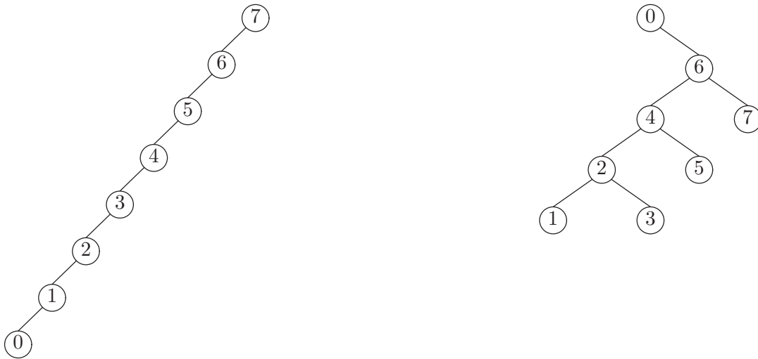
Figure 9.12: Splaying node 0 in a completely unbalanced tree. The resulting tree has about half the height of the original, speeding up subsequent searches.
