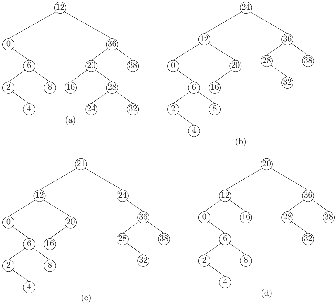
Figure 9.16: Basic BST operations on a splay tree. (a) is the original tree. (b) is the result of performing a splayFind on either of the values 21 or 24. (c) is the result of adding the value 21 into tree (a); the first step is to create the splayed tree (b). (d) is the result of removing 24 from the original tree (a); again the first step is to create (b), after which we splay the left child of 24 for the value 24, which is guaranteed to be larger than any value in that child.
