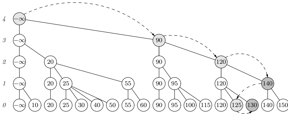
Figure 9.17: An abstract view of a skip list, showing its relationship to a (non-binary) search tree. Each key other than -\infty is duplicated to a random height. We can search this structure beginning at any level. In the best case, to search (unsuccessfully) for the target value 127, we need only look at the keys in the shaded nodes. Darker shaded nodes indicate keys larger than 127 that bound the search.
