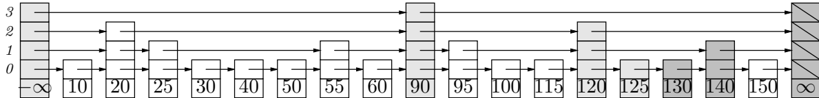
Figure 9.18: The skip list from Figure 9.17, showing a possible representation. The data structure is an ordered list whose nodes contain random numbers of pointers to later nodes (which allow intervening items in the list to be skipped during a search; hence the name). If a node has at least k pointers, then it contains a pointer to the next node that has at least k pointers. A node for \infty at the right allows us to avoid tests for null. Again, the nodes looked at during a search for 127 are shaded; the darker shading indicates nodes that limit the search.
